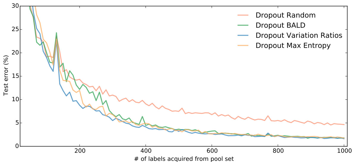
Fig. 5.2 Test error on MNIST as a function of number of labels acquired from the pool set. Four acquisition functions are shown ( Random , BALD , Variation Ratios , and Max Entropy ) evaluated with a Bernoulli approximating distribution ( Dropout ).
